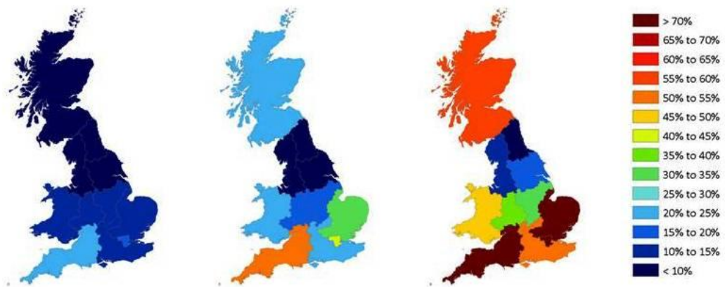
Figure 12 Regional response of the 200-year Loss to CS1 (left), CS2 (middle) and CS3 (right)
